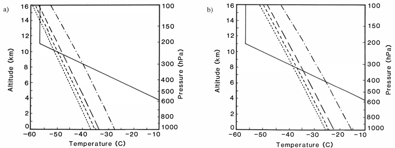
Fig. 4. Schmidt-Appleman diagram with threshold temperature T_{LC} versus altitude for relative humidity of 0 (short-dashed curve), 30 % (medium-dashed), 60 % (long-dashed) and 100 % (dash-dotted line), and the temperature profile of the international standard atmosphere (full). (a) For kerosene and overall propulsion efficiency of 0.3, (b) for hydrogen fuel and same efficiency.
