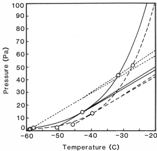
Fig. 7. As Fig. 3, according to the revised analysis, including the gradual conversion of kinetic energy into heat during mixing of the plumes with the environment. The straight mixing lines are for stagnant, the curved mixing lines with points for non-stagnant plumes.
