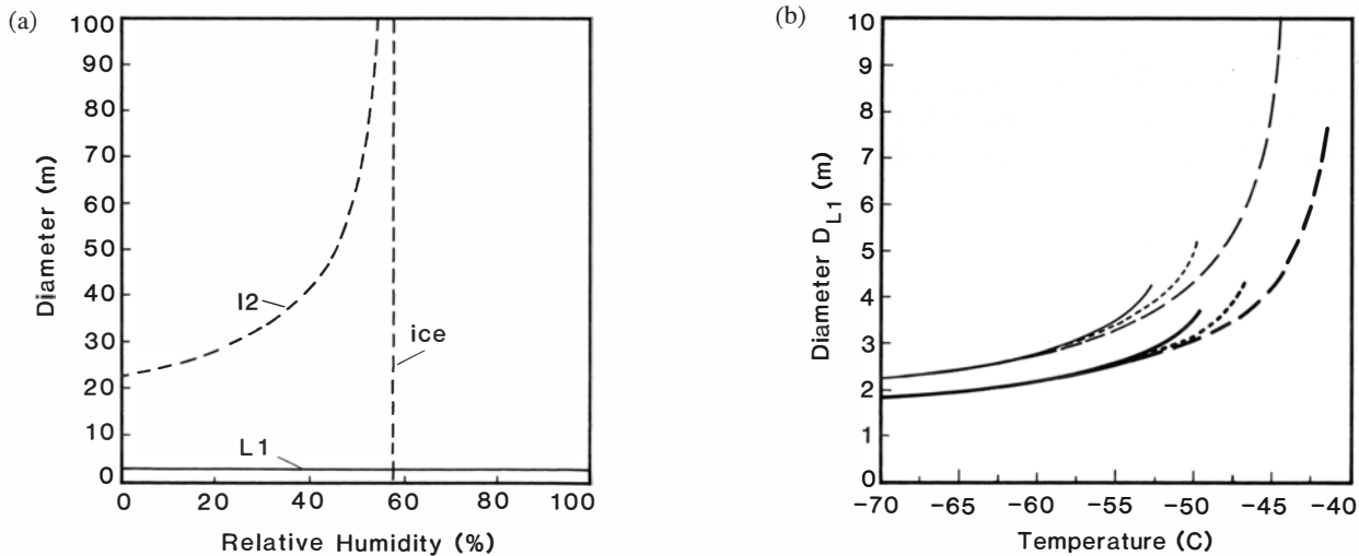
Fig. 6 (a). Contrail diameter at liquid saturation (L1) and at ice evaporation (I2) versus relative humidity under conditions as given in Table 2. For I2, \sqrt{2} D_{I2} is plotted as appropriate for a contrail formed by two jet engines. The vertical dashed line indicates ice saturation humidity. (b) Diameter D L1 versus temperature T E for conditions as in Table 2 (220 hPa, upper, thin curves) and at 300 hPa (lower, thick curves), for three ambient humidity conditions: totally dry (full), ice saturation (short-dashed), and water saturation (long-dashed).
